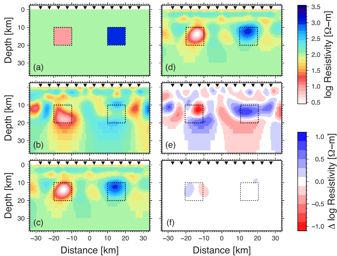
Figure 1. (a) A synthetic 2-D model comprising two square regions of 10 and 1000 \Omega\text{-m} resistivity embedded within a 100 \Omega\text{-m} halfspace, (b) the model obtained by inverting the synthetic data with 3 per cent Gaussian noise and 10 per cent additive Cauchy-distributed noise for contamination, as described in the text, (c) the model obtained by inverting the culled data set at the second (final) robust run, (d) the model obtained by inverting the synthetic data with only the 3 per cent Gaussian noise, (e) the difference in logarithmic resistivity between the two models in (b) and (d), and (f) the difference in logarithmic resistivity between the two models in (c) and (d). The dashed squares in the figures indicate the location of the two square regions in the synthetic model of (a). The inverted triangles at the top of the models denote the site locations. In all of the inversions, the regularization parameter for model smoothness \tau_s was 1, and the weighting factors for model smoothness \alpha and \beta were 1 and 3, respectively.
